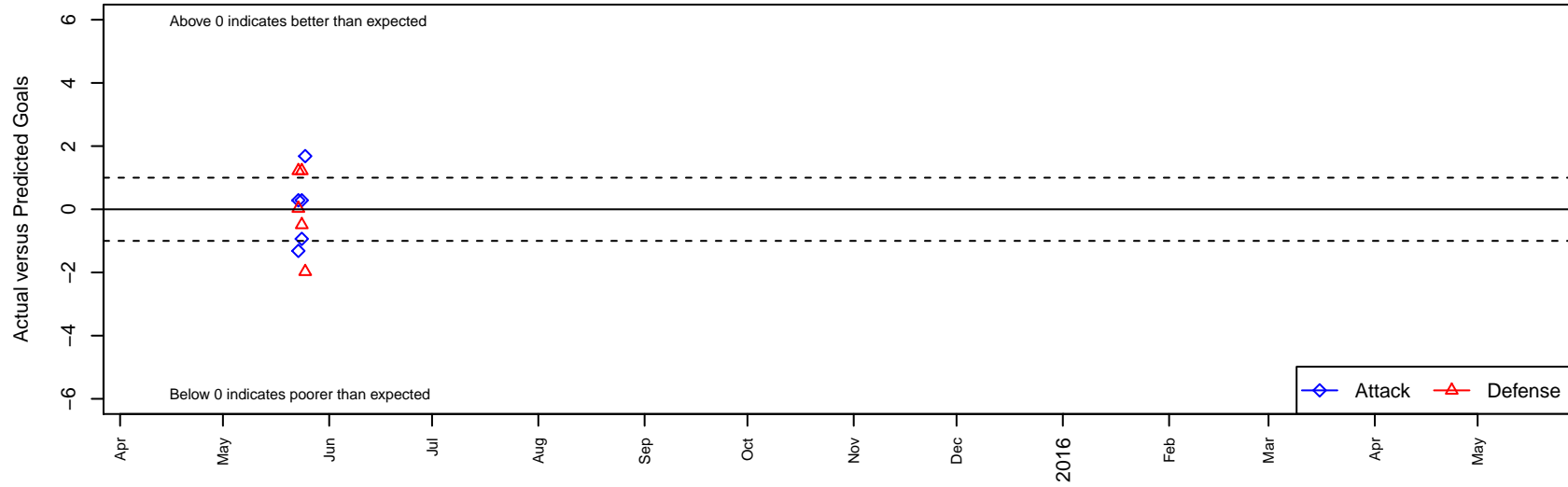
ARFC 03 Freedom G02 Dots are actual minus expected GF (blue circles) and GA (red triangles). Blue line is smoothed change in attack strength. Red is smoothed change in defense strength.
